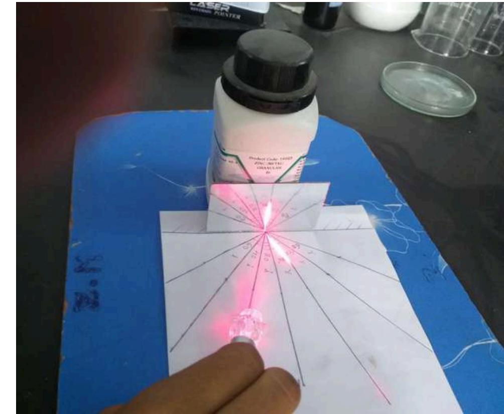
Verification of laws of reflection
